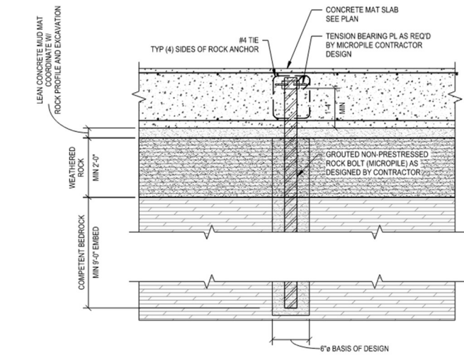
TYPICAL ROCK ANCHOR DETAIL A S-3-2 NOT TO SCALE
